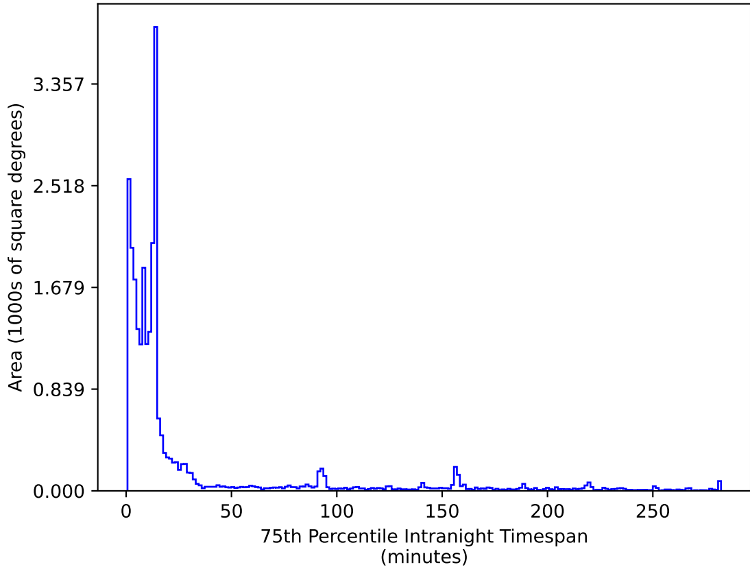
noroll_v3.4_10yrs All sky i band: 75th Percentile Intranight Timespan
