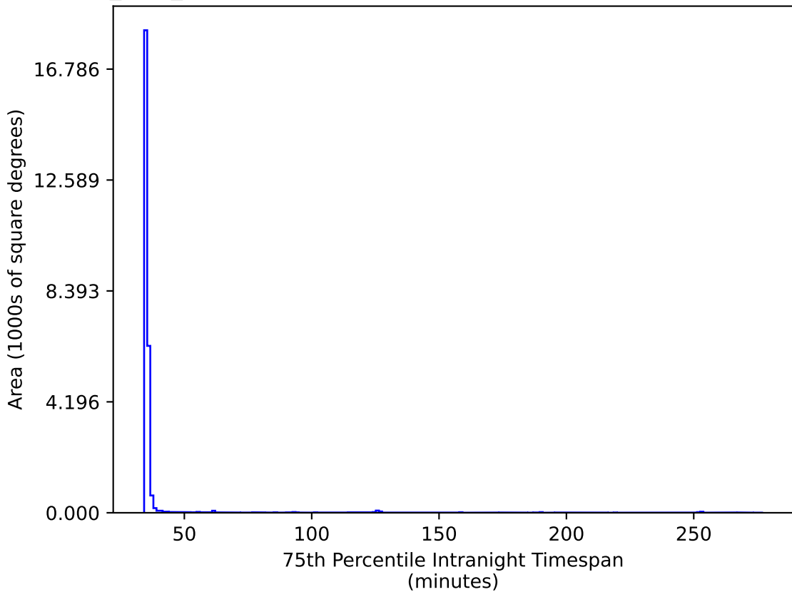
noroll_v3.4_10yrs All sky gr bands: 75th Percentile Intranight Timespan
