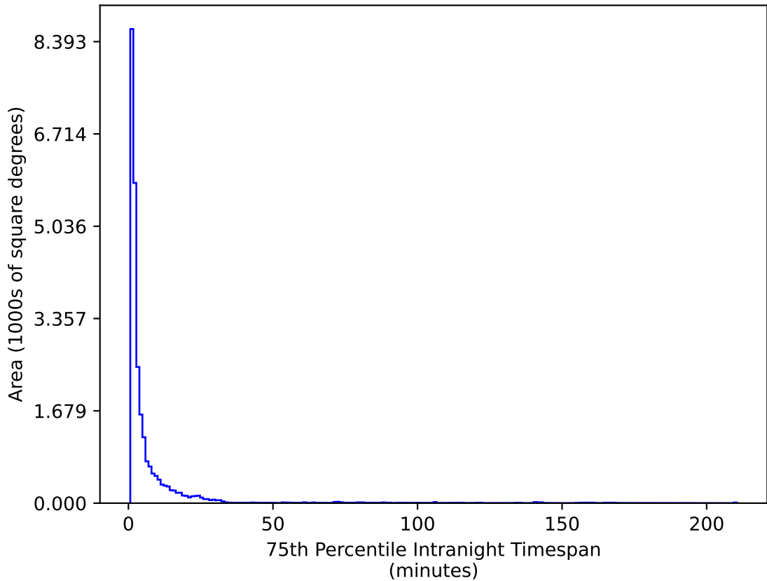
noroll_v3.4_10yrs All sky g band: 75th Percentile Intranight Timespan
