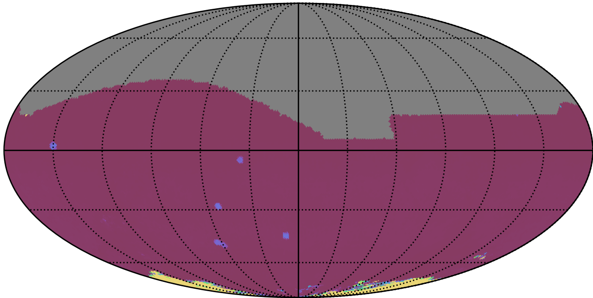
noroll_v3.4_10yrs All sky: 75th Percentile Intranight Timespan
