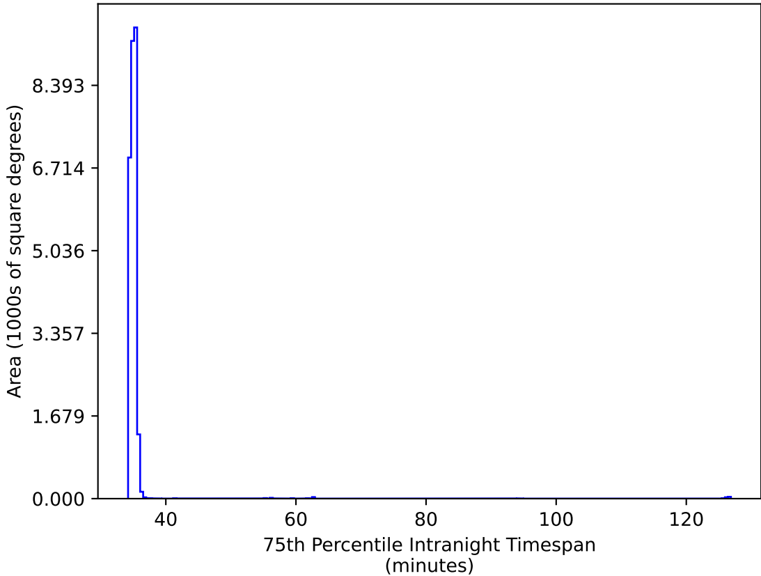
noroll_v3.4_10yrs All sky: 75th Percentile Intranight Timespan
