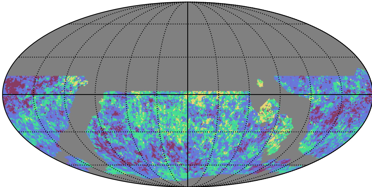
noroll_v3.4_10yrs WFD z band: 20thPercentile Inter-Night Gap
