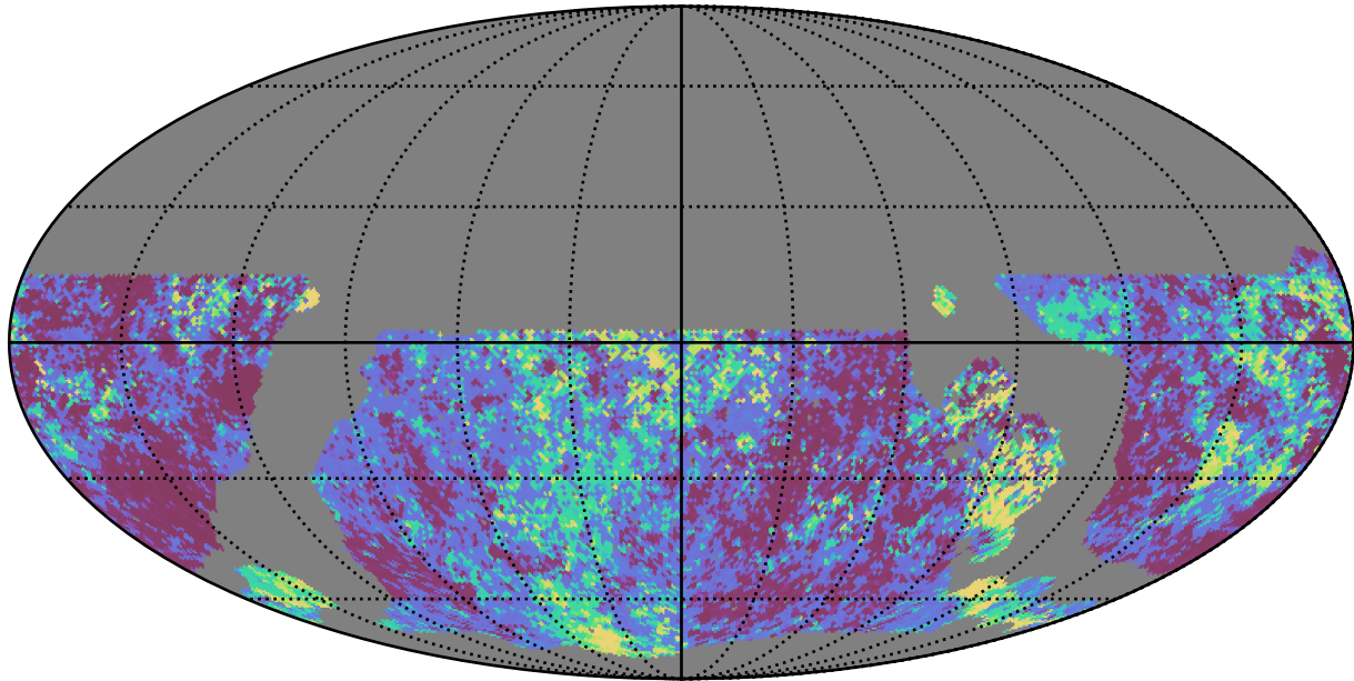
noroll_v3.4_10yrs WFD y band: 20thPercentile Inter-Night Gap
