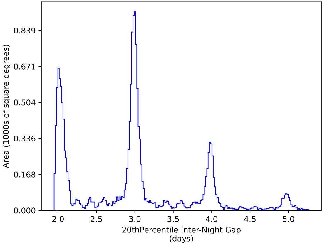
noroll_v3.4_10yrs WFD y band: 20thPercentile Inter-Night Gap
