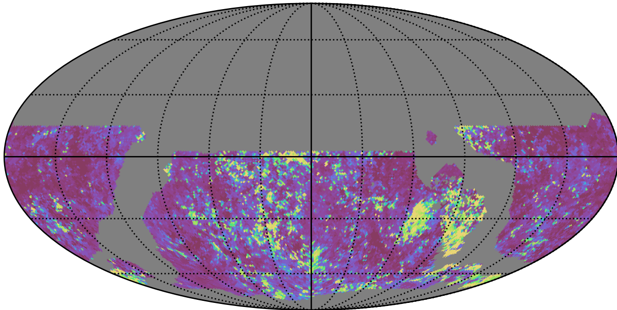
noroll_v3.4_10yrs WFD u band: 20thPercentile Inter-Night Gap
