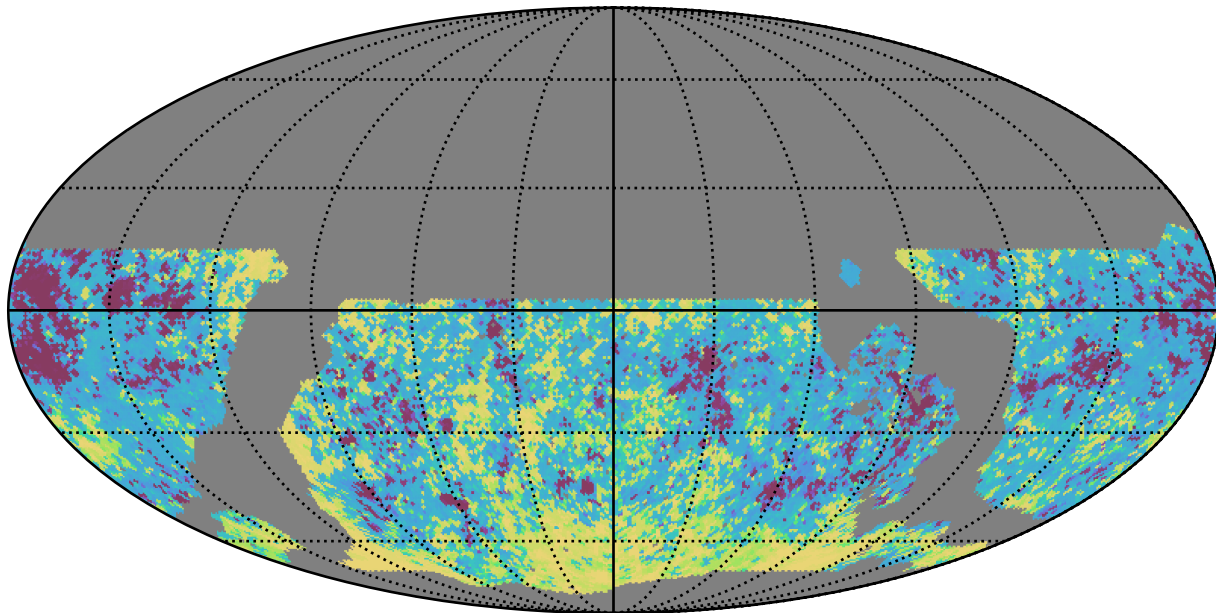
noroll_v3.4_10yrs WFD i band: 20thPercentile Inter-Night Gap
