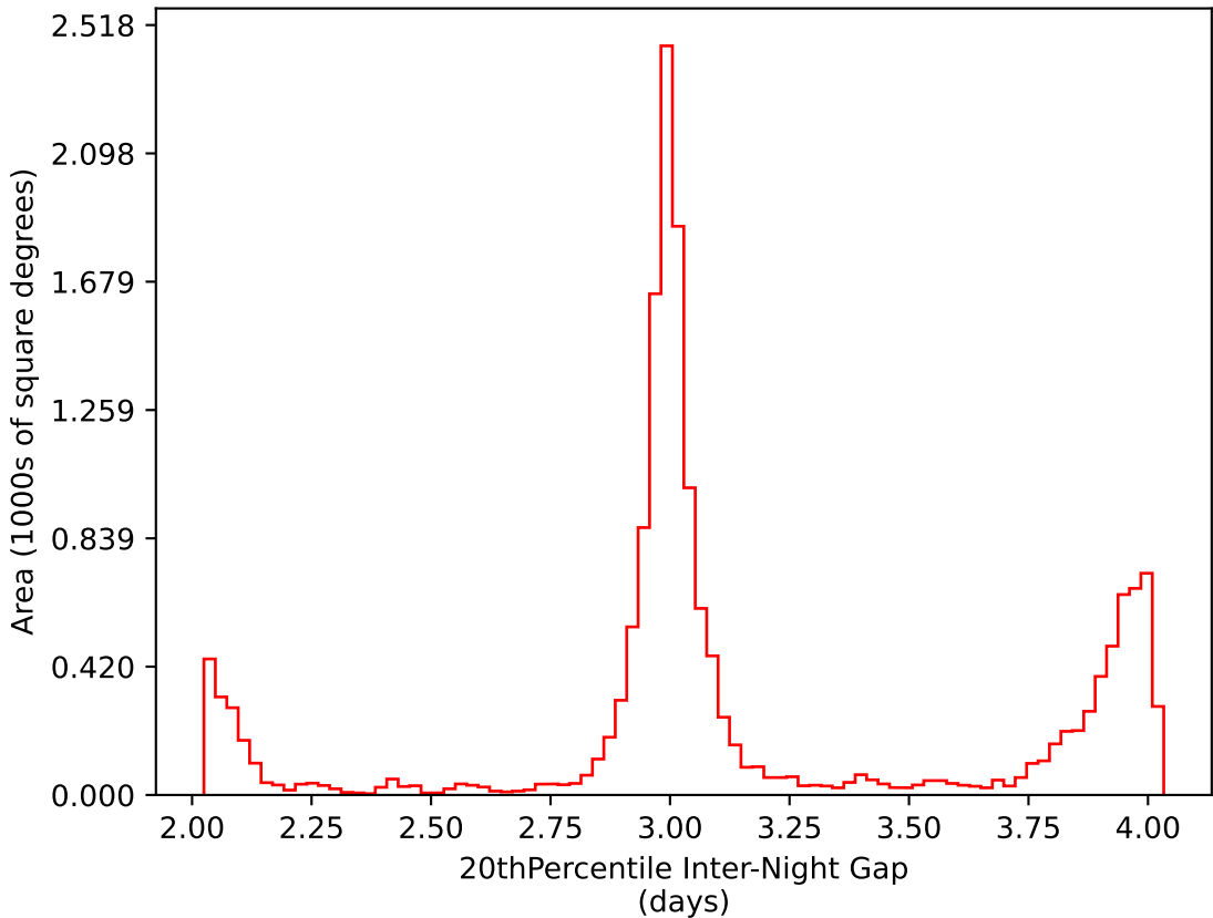
noroll_v3.4_10yrs WFD i band: 20thPercentile Inter-Night Gap
