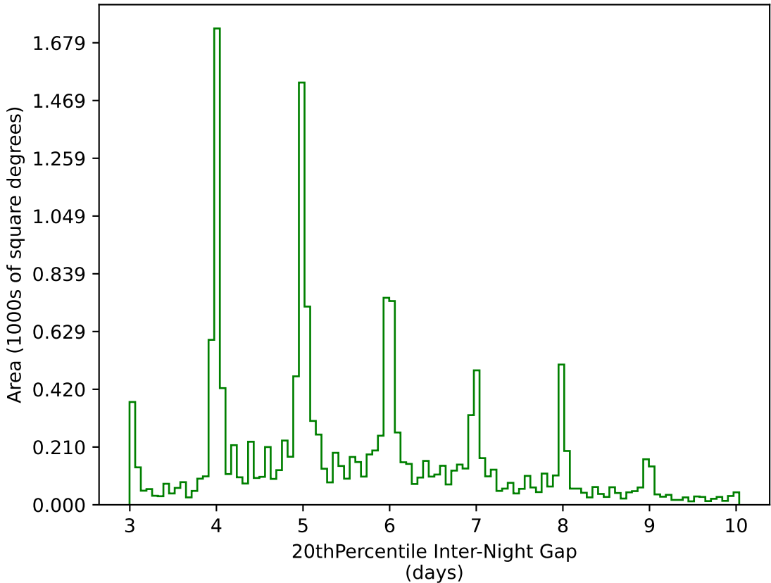
noroll_v3.4_10yrs WFD g band: 20thPercentile Inter-Night Gap
