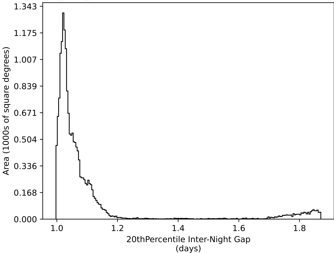
noroll_v3.4_10yrs WFD all bands: 20thPercentile Inter-Night Gap
