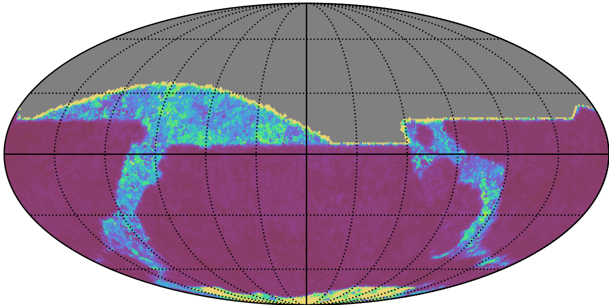
noroll_v3.4_10yrs All sky z band: 20thPercentile Inter-Night Gap
