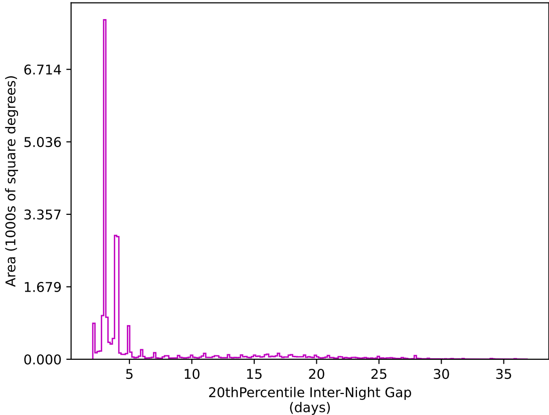
noroll_v3.4_10yrs All sky z band: 20thPercentile Inter-Night Gap
