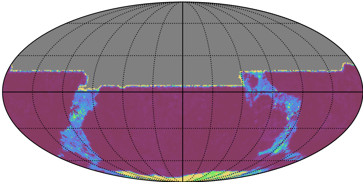
noroll_v3.4_10yrs All sky y band: 20thPercentile Inter-Night Gap
