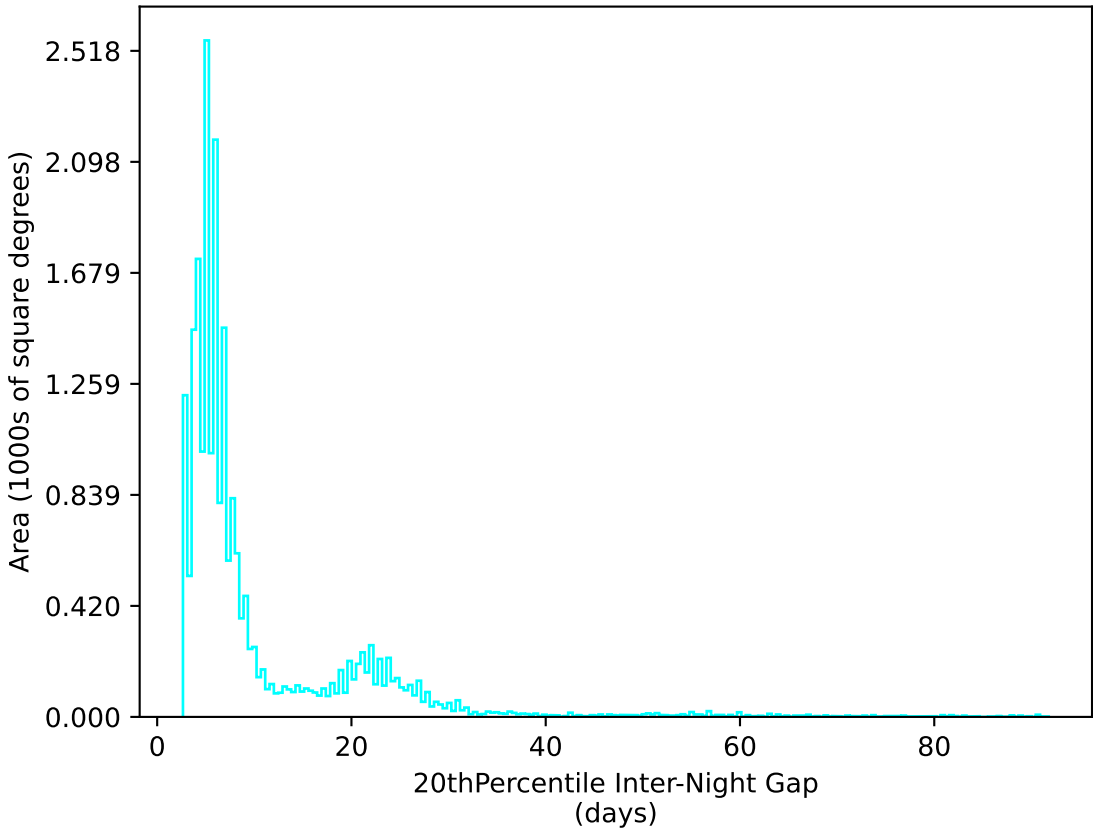
noroll_v3.4_10yrs All sky u band: 20thPercentile Inter-Night Gap
