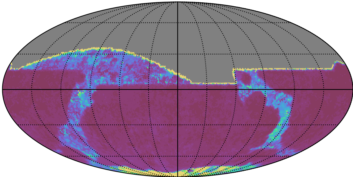
noroll_v3.4_10yrs All sky r band: 20thPercentile Inter-Night Gap
