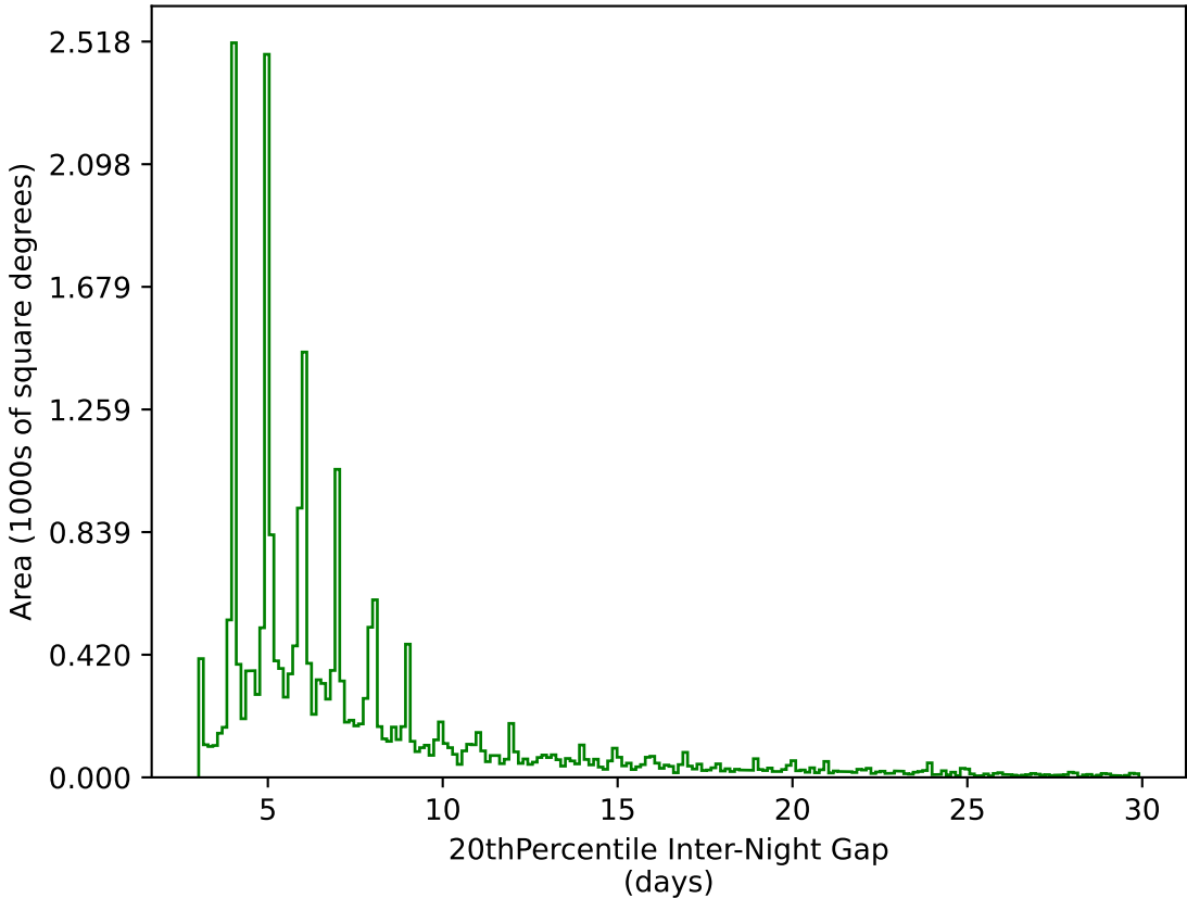
noroll_v3.4_10yrs All sky g band: 20thPercentile Inter-Night Gap
