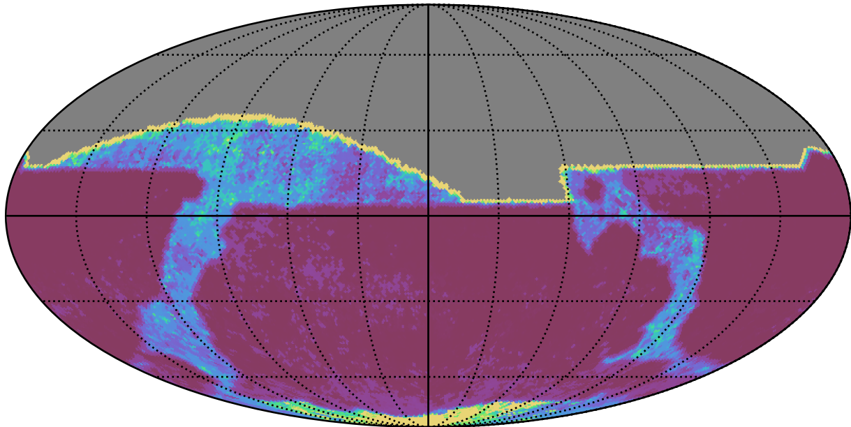
noroll_v3.4_10yrs All sky all bands: 20thPercentile Inter-Night Gap
