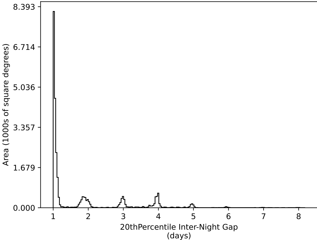
noroll_v3.4_10yrs All sky all bands: 20thPercentile Inter-Night Gap
