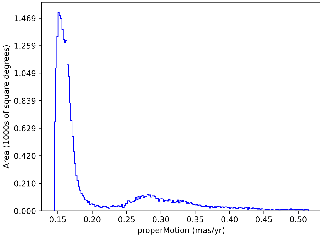
noroll_v3.4_10yrs : properMotion
