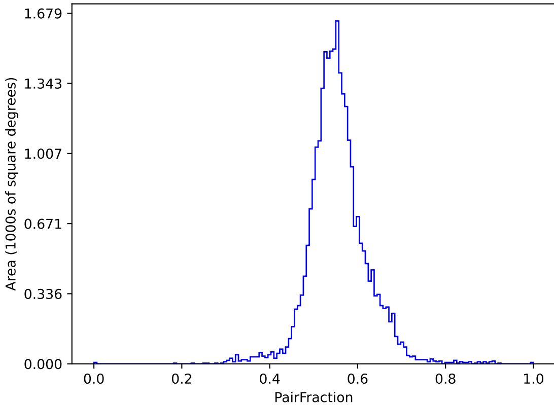
noroll_v3.4_10yrs (g or r or i): PairFraction
