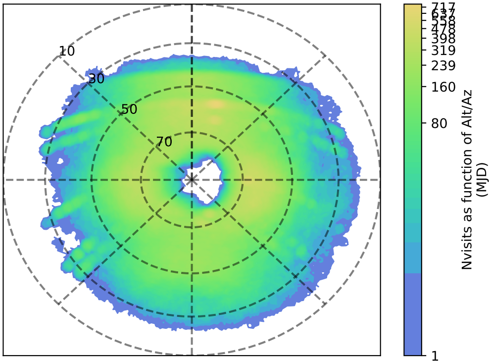
noroll_v3.4_10yrs u: Nvisits as function of Alt/Az
