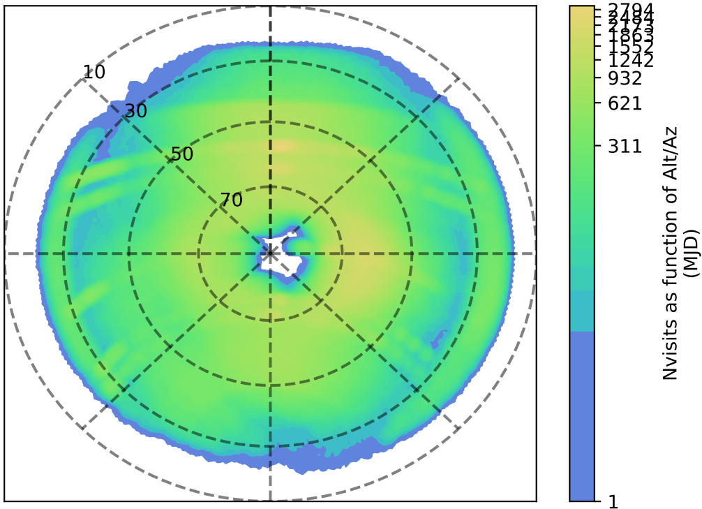
noroll_v3.4_10yrs i: Nvisits as function of Alt/Az
