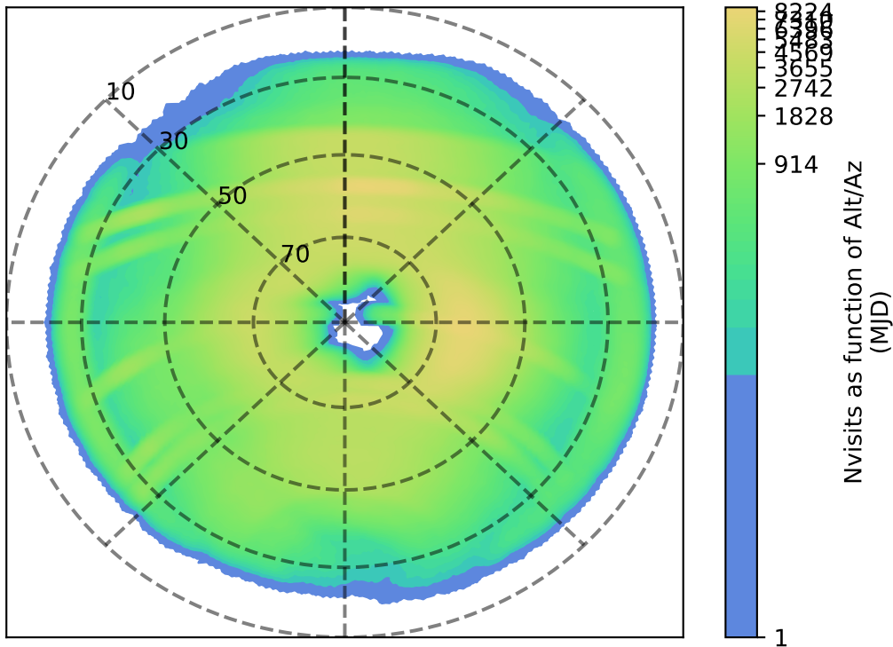
noroll_v3.4_10yrs : Nvisits as function of Alt/Az
