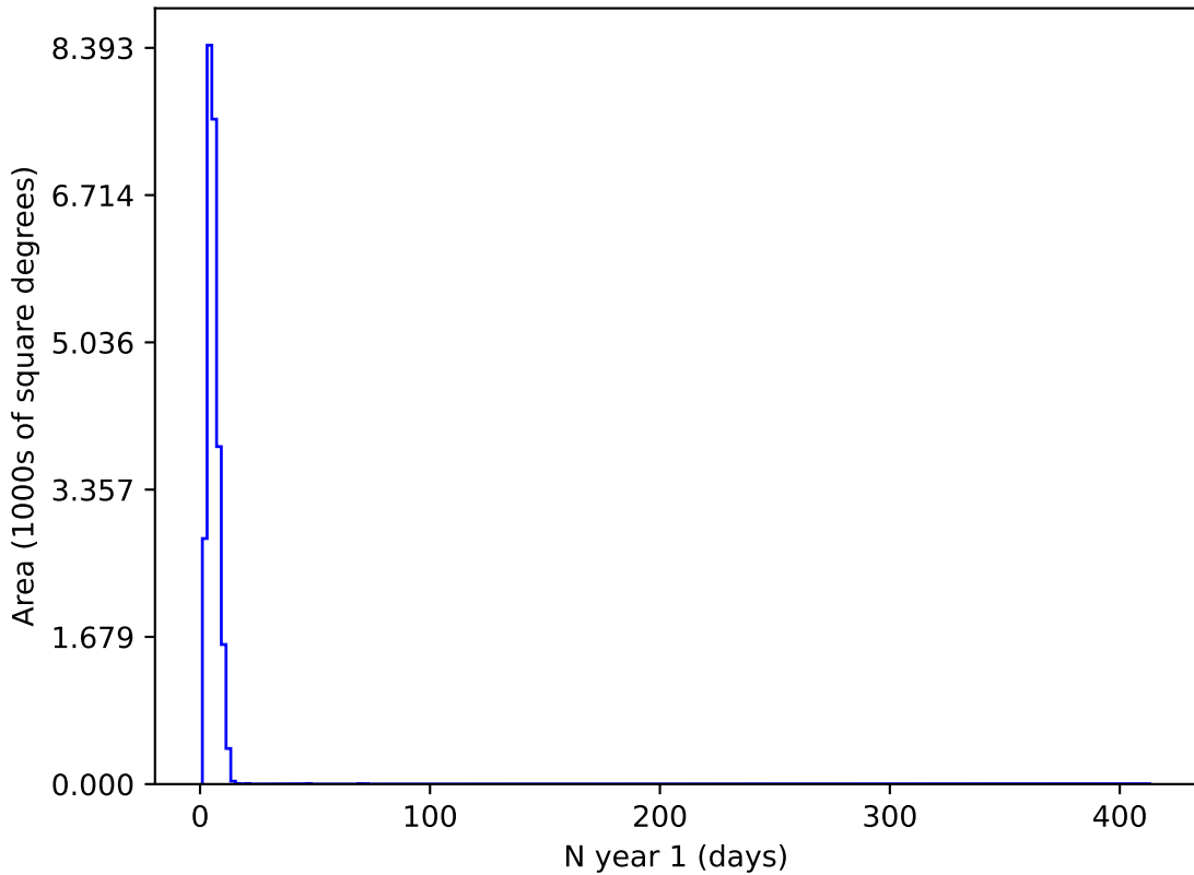
noroll_v3.4_10yrs u and night < 365: N year 1
