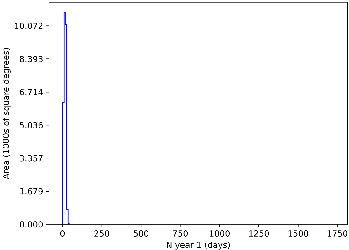
noroll_v3.4_10yrs r and night < 365: N year 1
