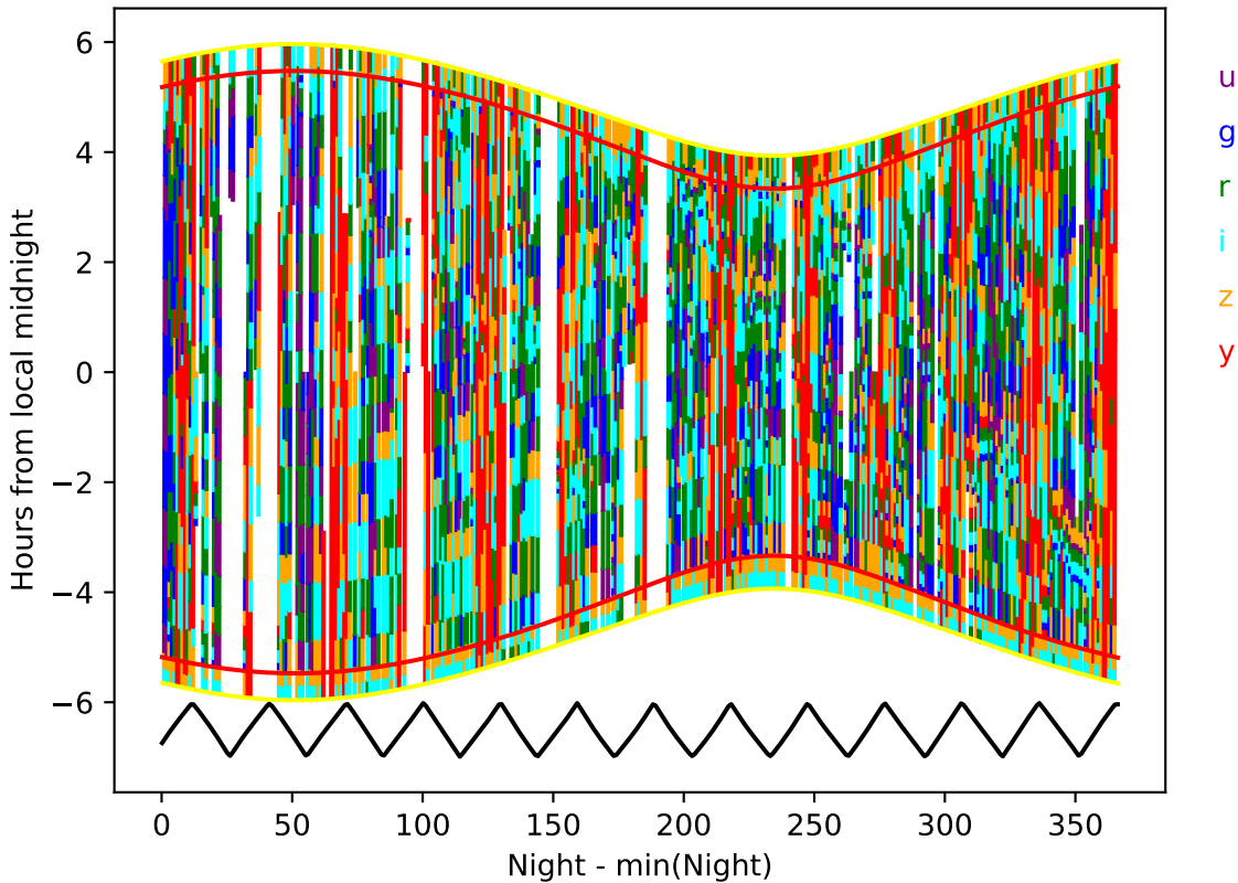
noroll_v3.4_10yrs year 0-1: Hourglass
