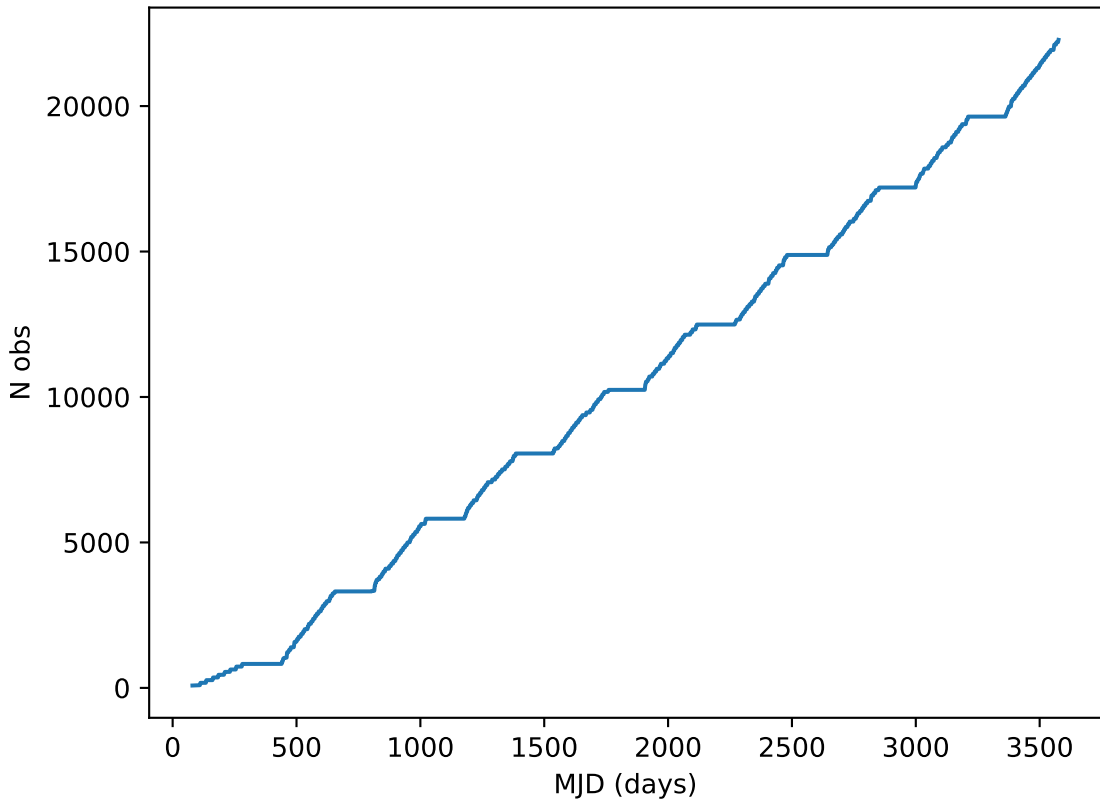
noroll_v3.4_10yrs note like DD:XMM_LSS%: Cumulative
