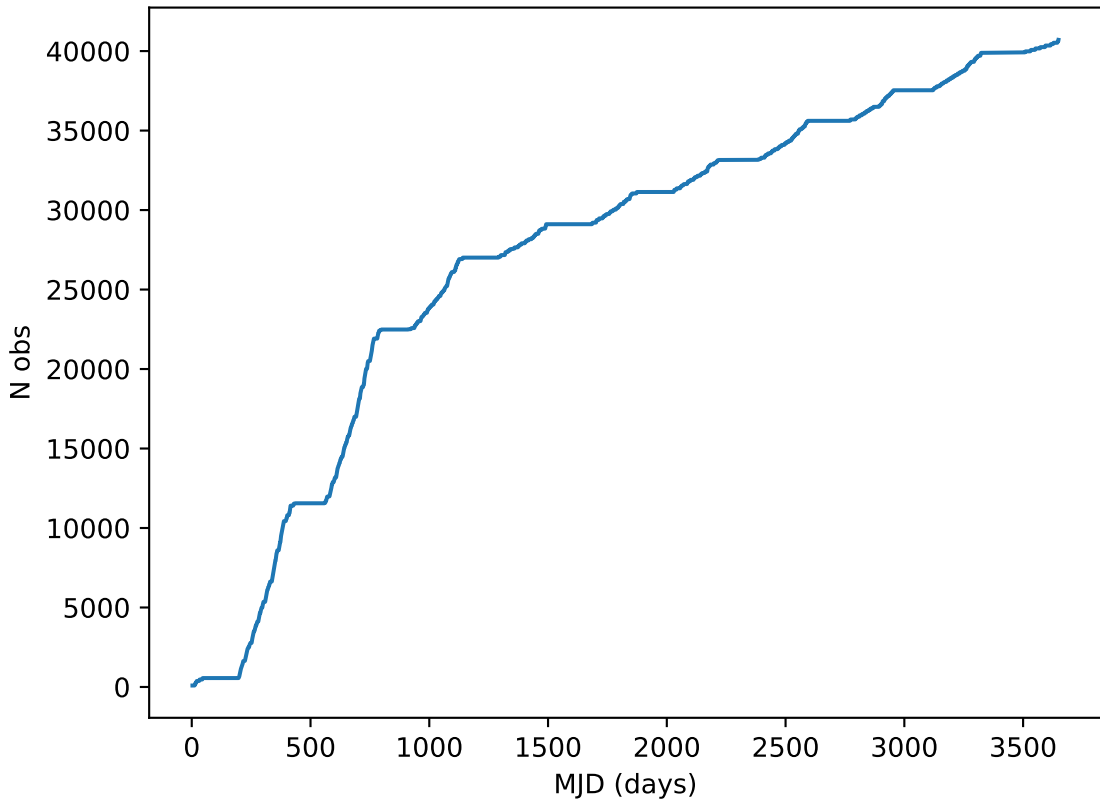
noroll_v3.4_10yrs note like DD: COSMOS%: Cumulative
