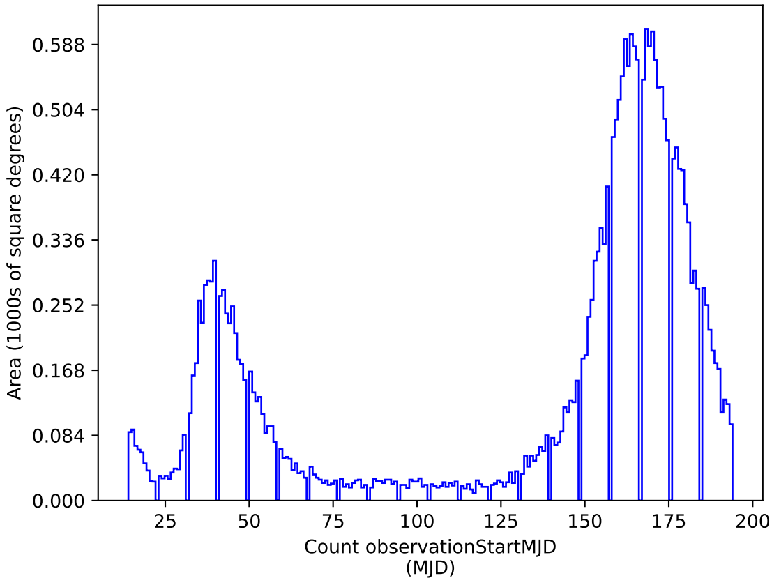
noroll_v3.4_10yrs z: Count observationStartMJD
