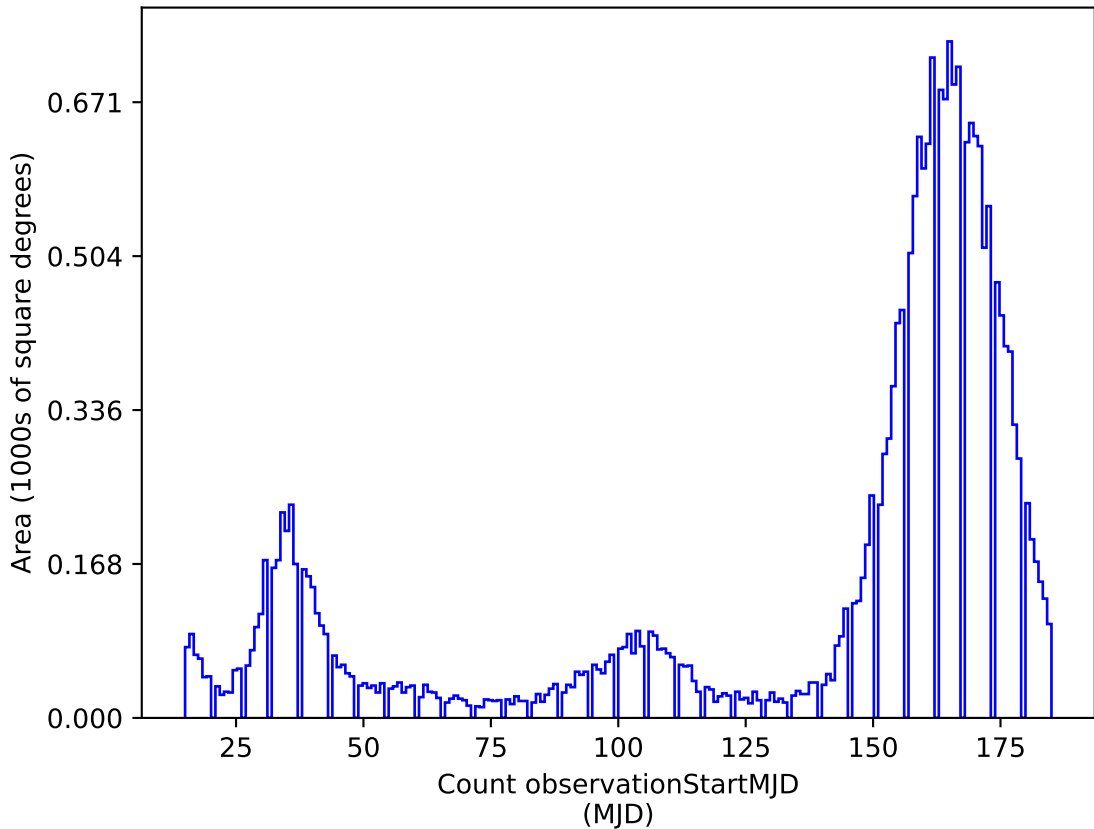
noroll_v3.4_10yrs y: Count observationStartMJD
