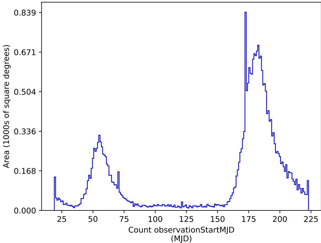
noroll_v3.4_10yrs r: Count observationStartMJD
