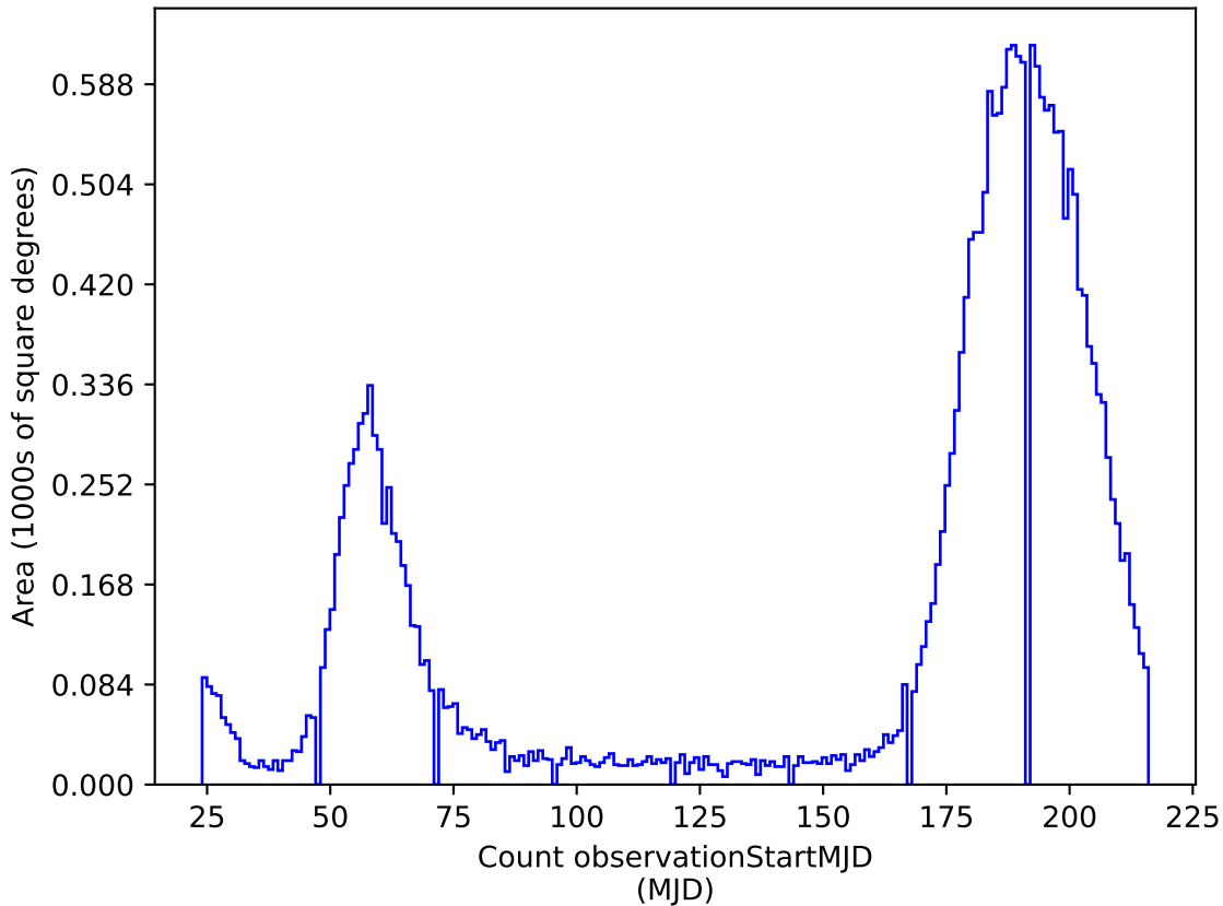
noroll_v3.4_10yrs i: Count observationStartMJD
