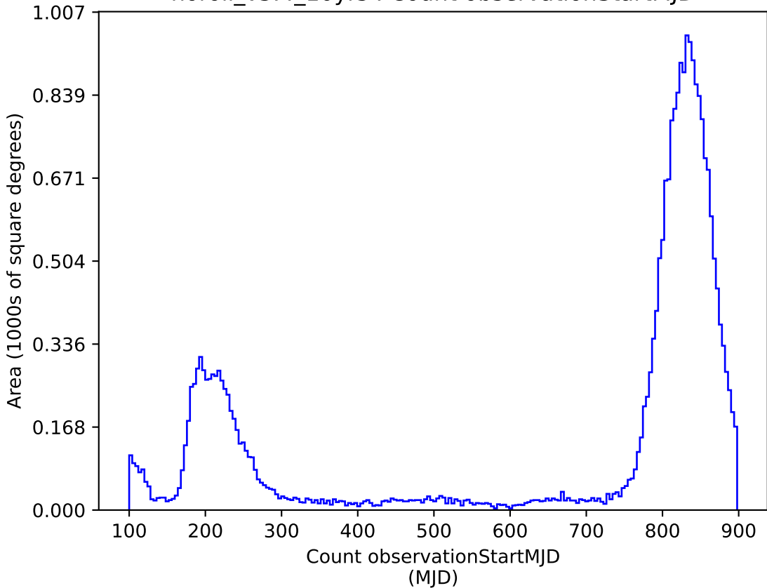
noroll_v3.4_10yrs : Count observationStartMJD
