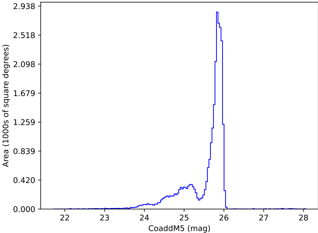
noroll_v3.4_10yrs z: CoaddM5
