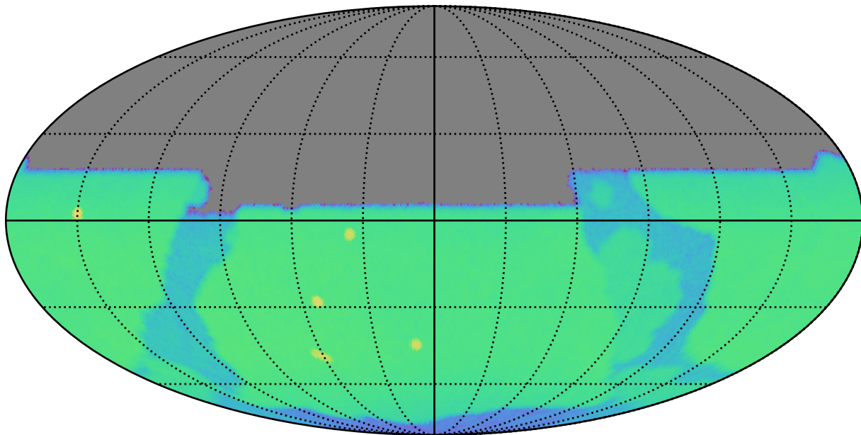
noroll_v3.4_10yrs y: CoaddM5
