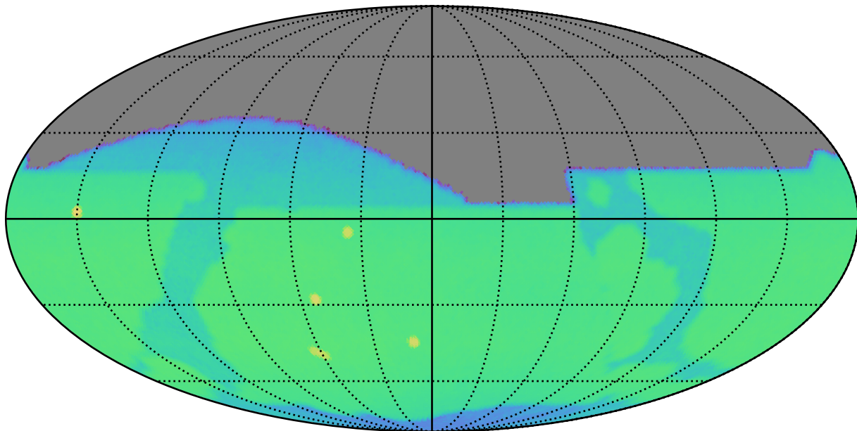
noroll_v3.4_10yrs r: CoaddM5
