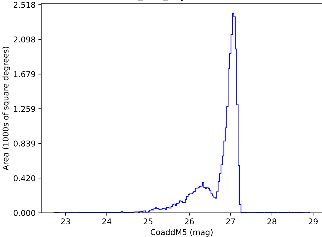
noroll_v3.4_10yrs r: CoaddM5
