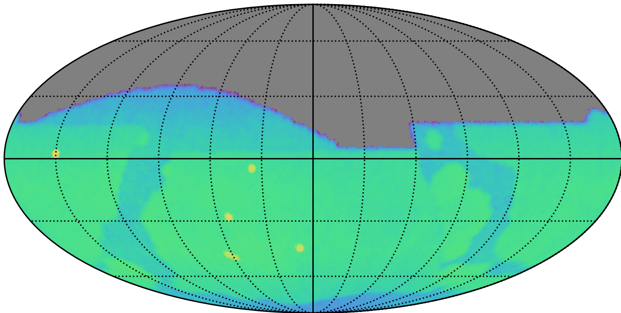
noroll_v3.4_10yrs g: CoaddM5
