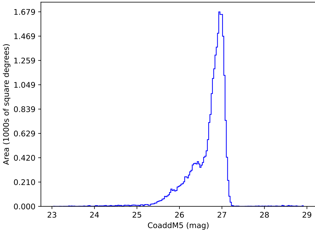
noroll_v3.4_10yrs g: CoaddM5
