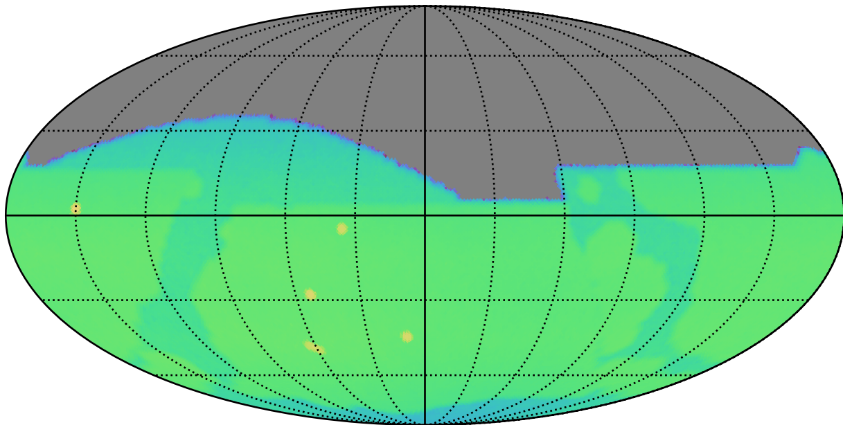
noroll_v3.4_10yrs : CoaddM5
