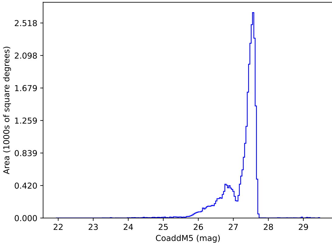
noroll_v3.4_10yrs : CoaddM5
