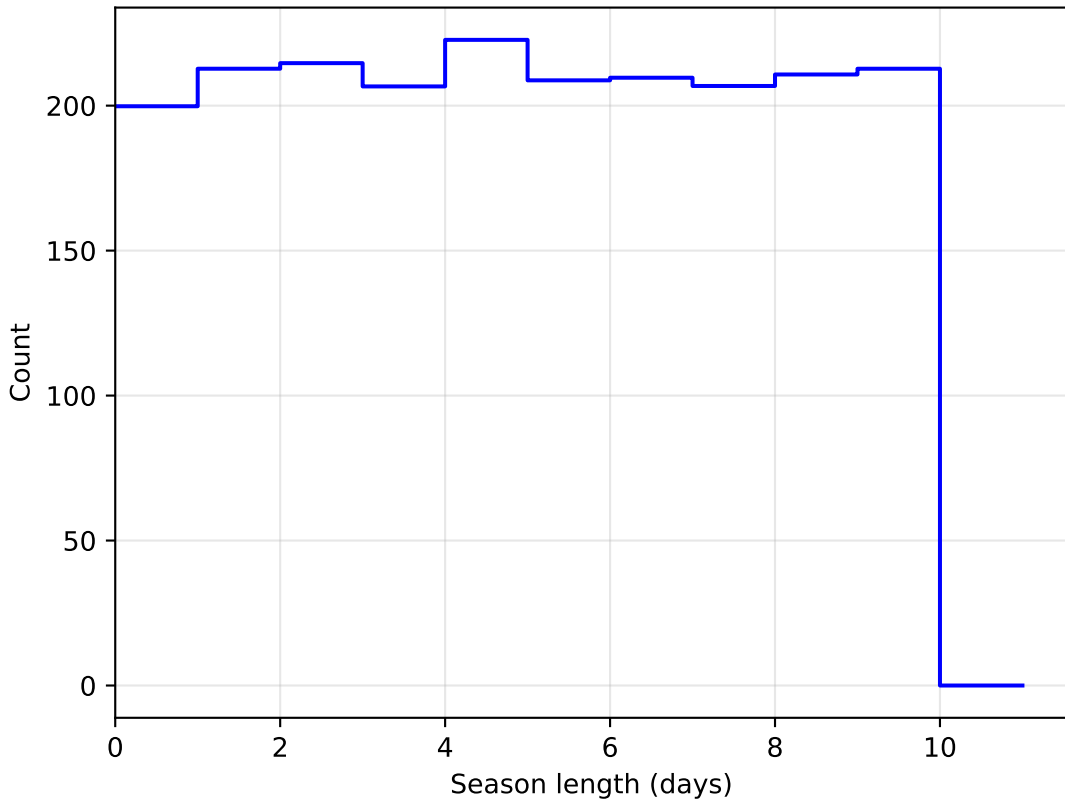
noroll_v3.4_10yrs DD:XMM_LSS all bands: SeasonLength
