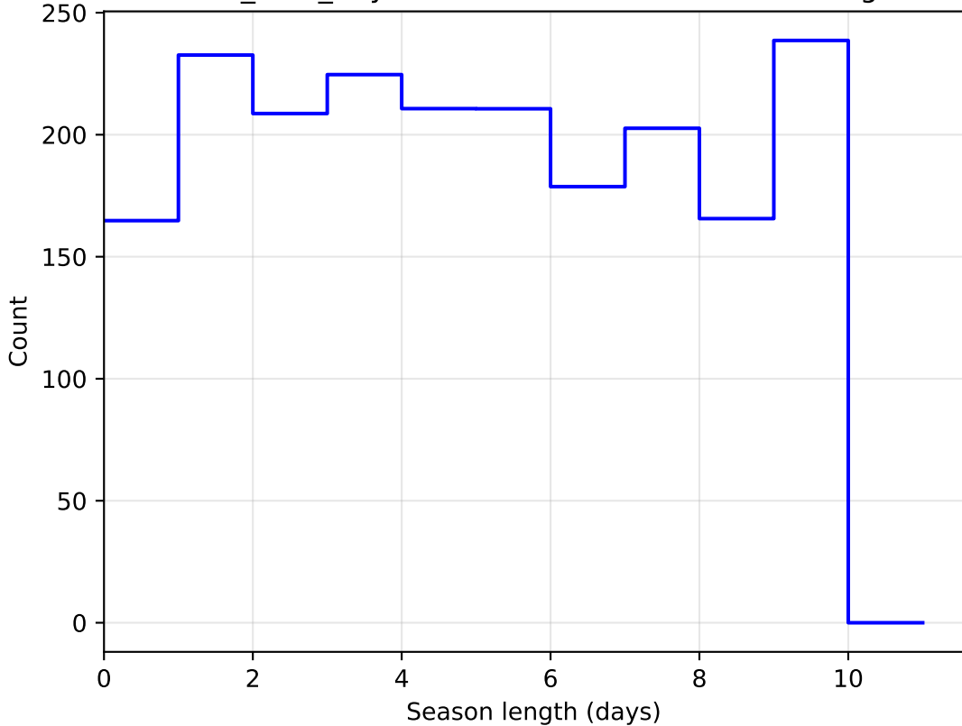
noroll_v3.4_10yrs DD:WFD all bands: SeasonLength
