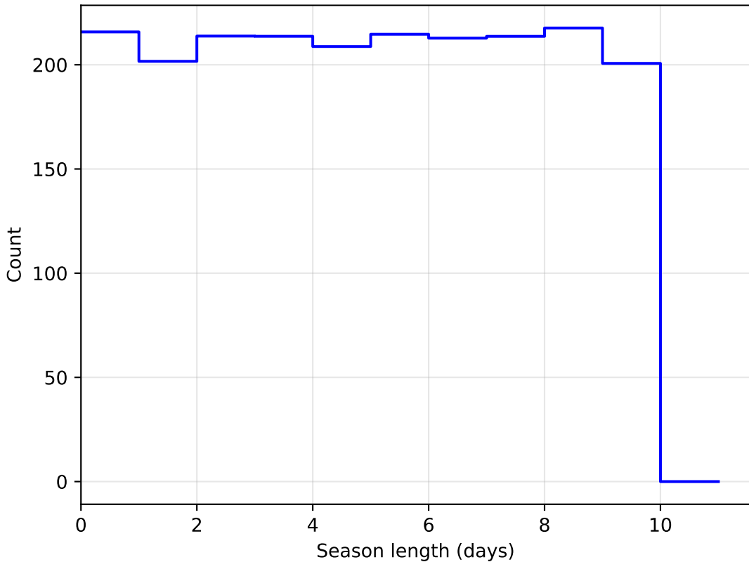
noroll_v3.4_10yrs DD:ECDFS all bands: SeasonLength
