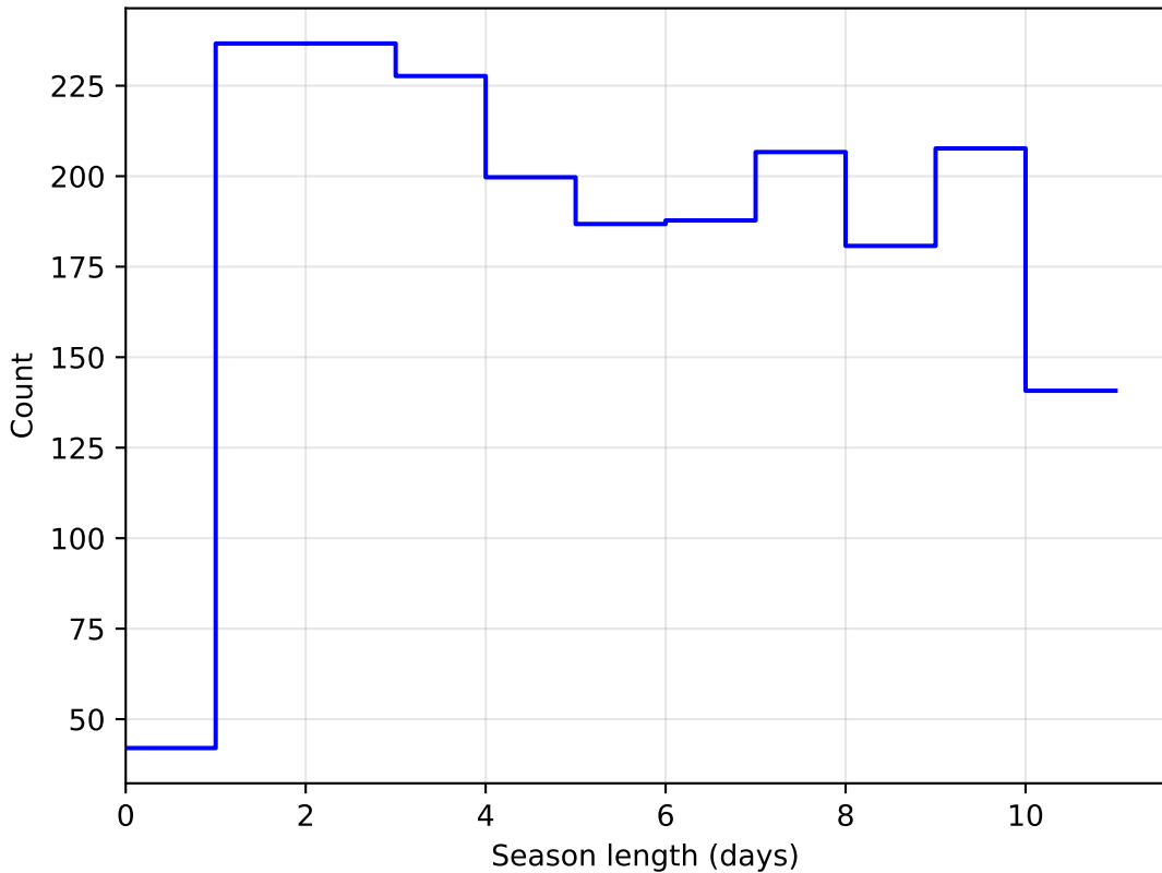
noroll_v3.4_10yrs DD: COSMOS all bands: SeasonLength
