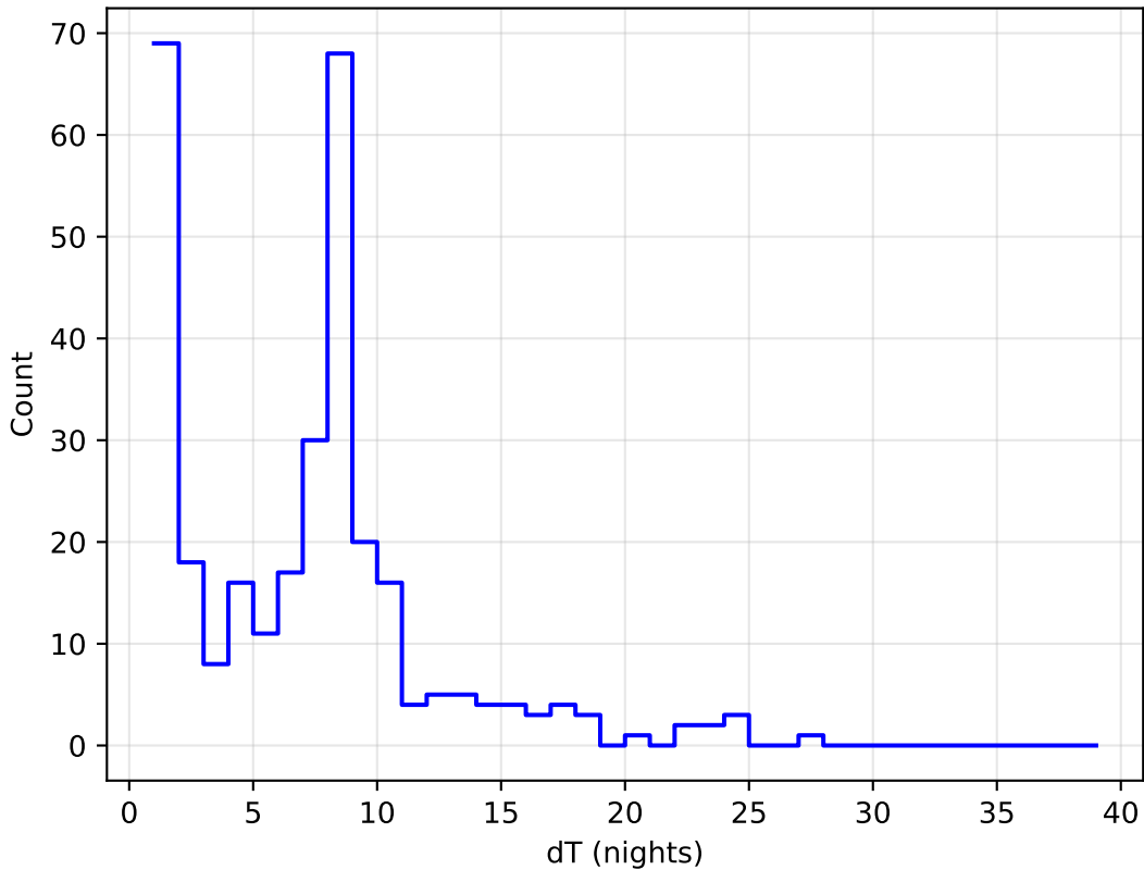
noroll_v3.4_10yrs all bands: DD:XMM_LSS Delta Nights Histogram
