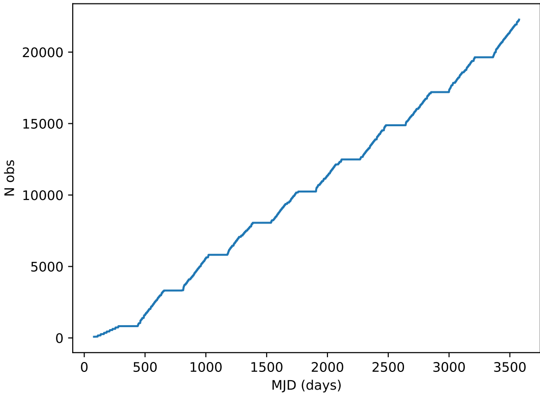
noroll_v3.4_10yrs all bands: DD:XMM_LSS Cumulative NVisits
